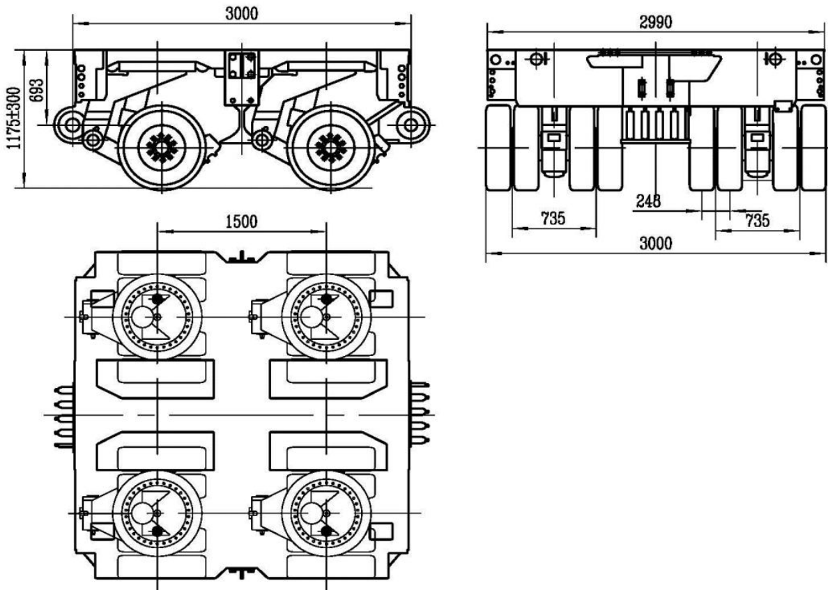
Three axle-lines Modular Multi-axle trailer
