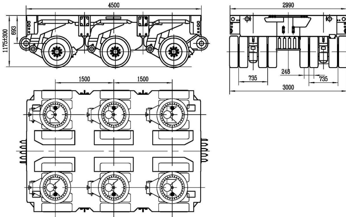
Four axle-lines Modular Multi-axle trailer
