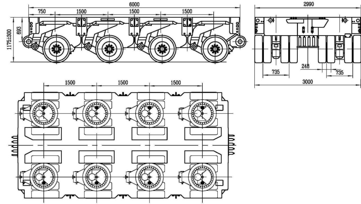
Five axle-lines Modular Multi-axle trailer
