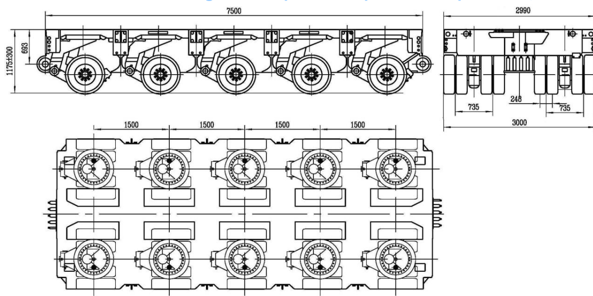
Six axle-lines Modular Multi-axle trailer
